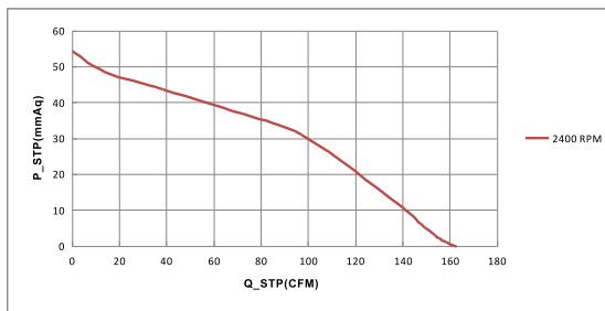
P&amp;Q曲线(在额定电压下) P&amp;Q CURVE (AT RATEDVOLTAGE)
